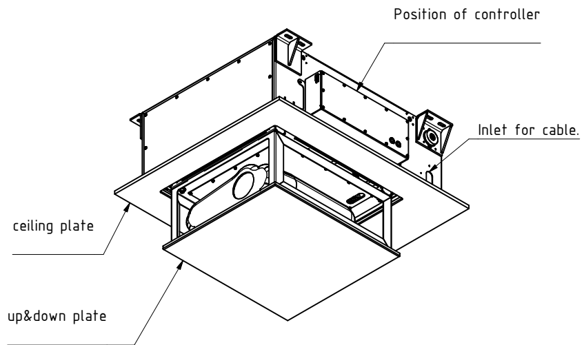
Mounting Frame (Option) Surface: powder-coated in RAL9005 fine
